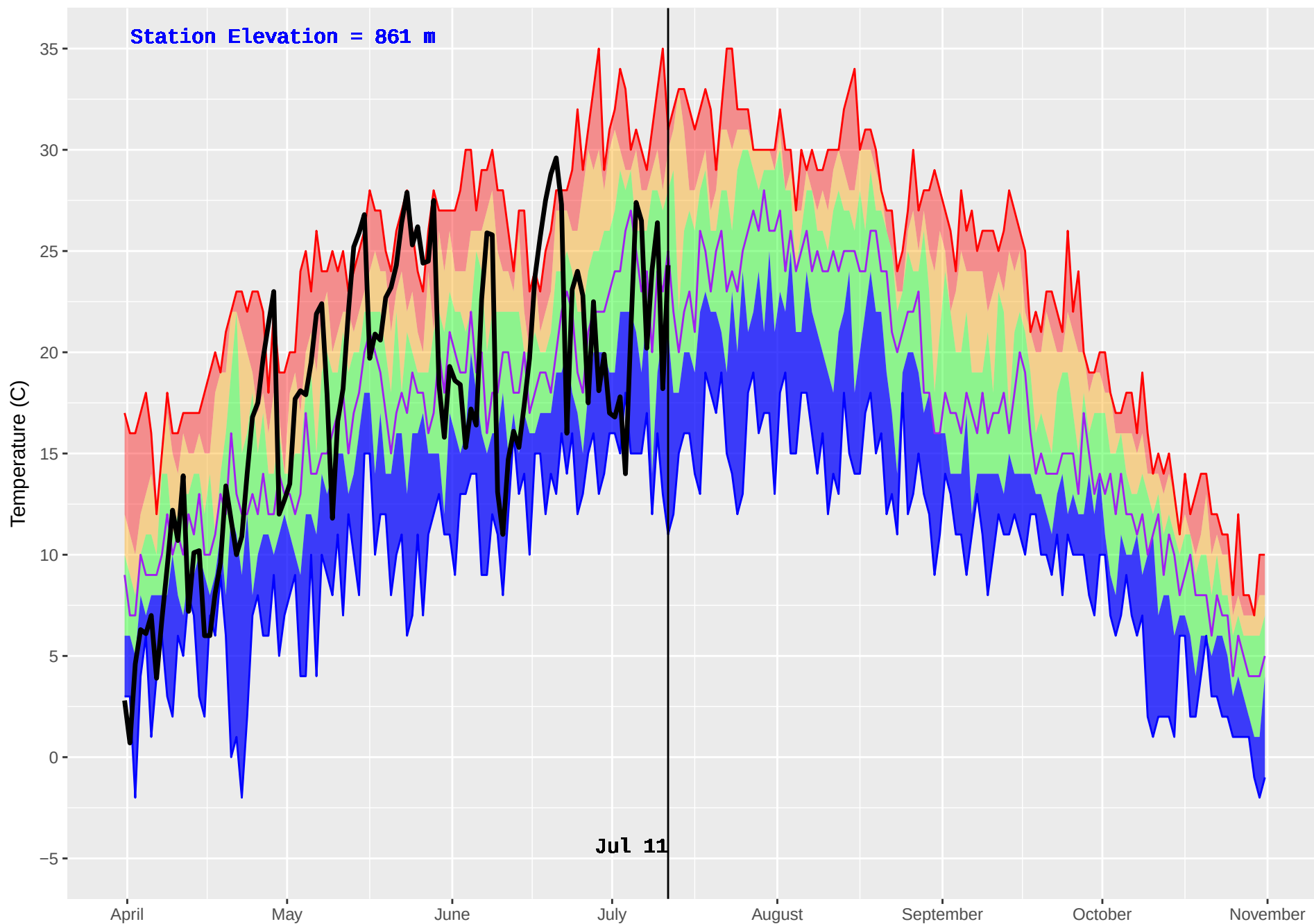
BLAEBERRY (866) : Historical (2004–2016) and Current (2018) Noon Temperature
