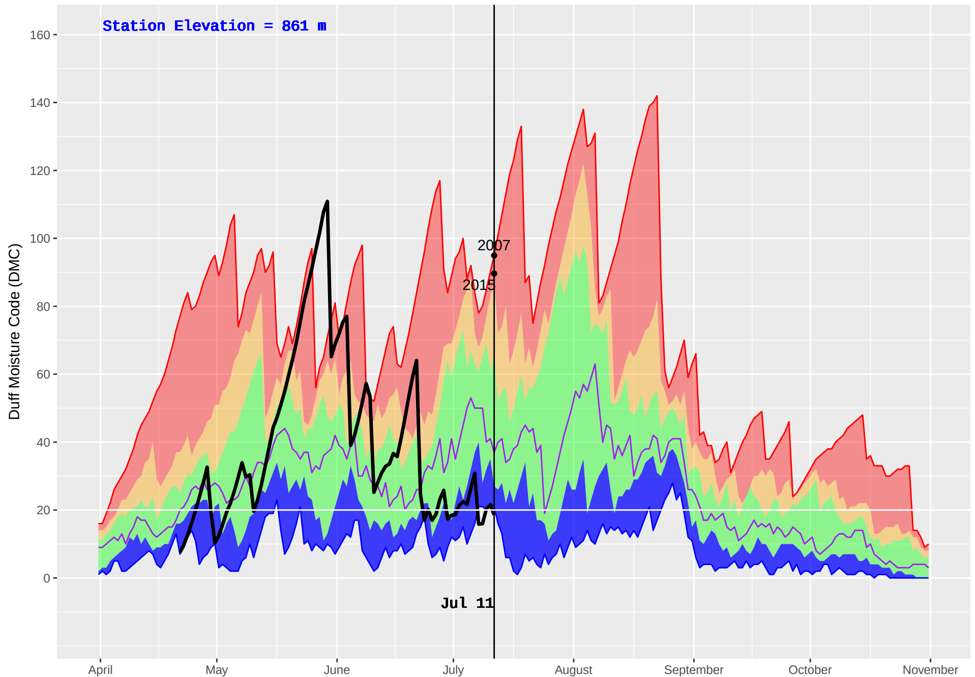
BLAEBERRY (866) : Historical (2004–2016) and Current (2018) Noon Duff Moisture Code (DMC)
