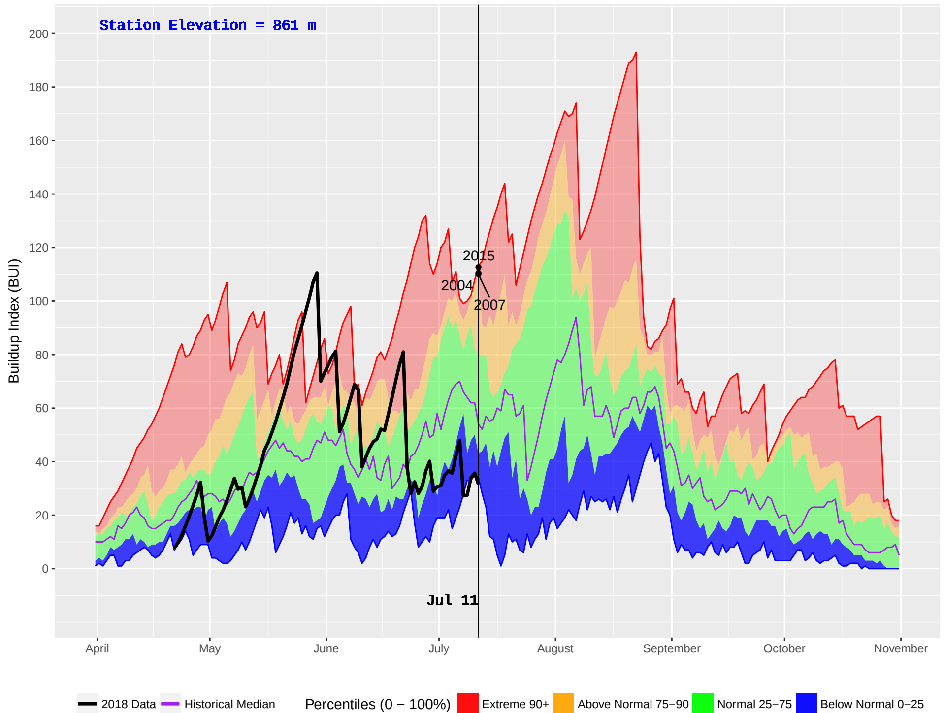
BLAEBERRY (866) : Historical (2004–2016) and Current (2018) Noon Buildup Index (BUI)
