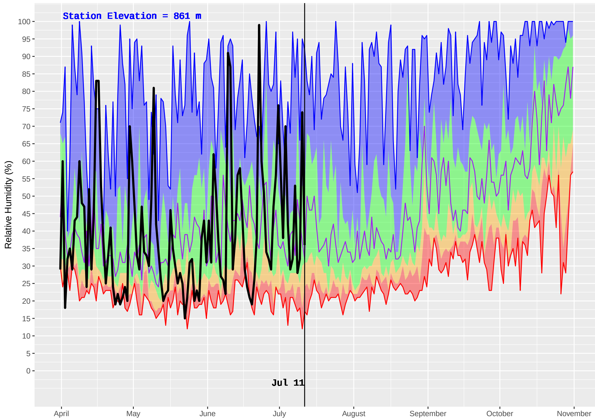
BLAEBERRY (866) : Historical (2004–2016) and Current (2018) Noon Relative Humidity
